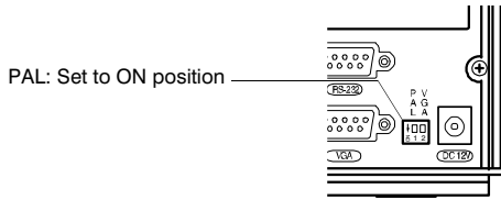
Figure 2-1 NTSC/PAL Operation Switch
